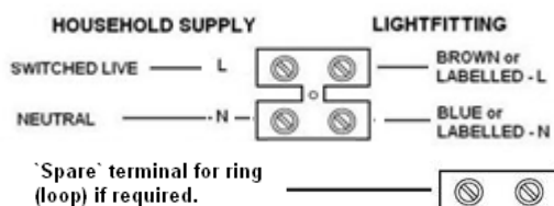
④ Details of terminal wiring.
